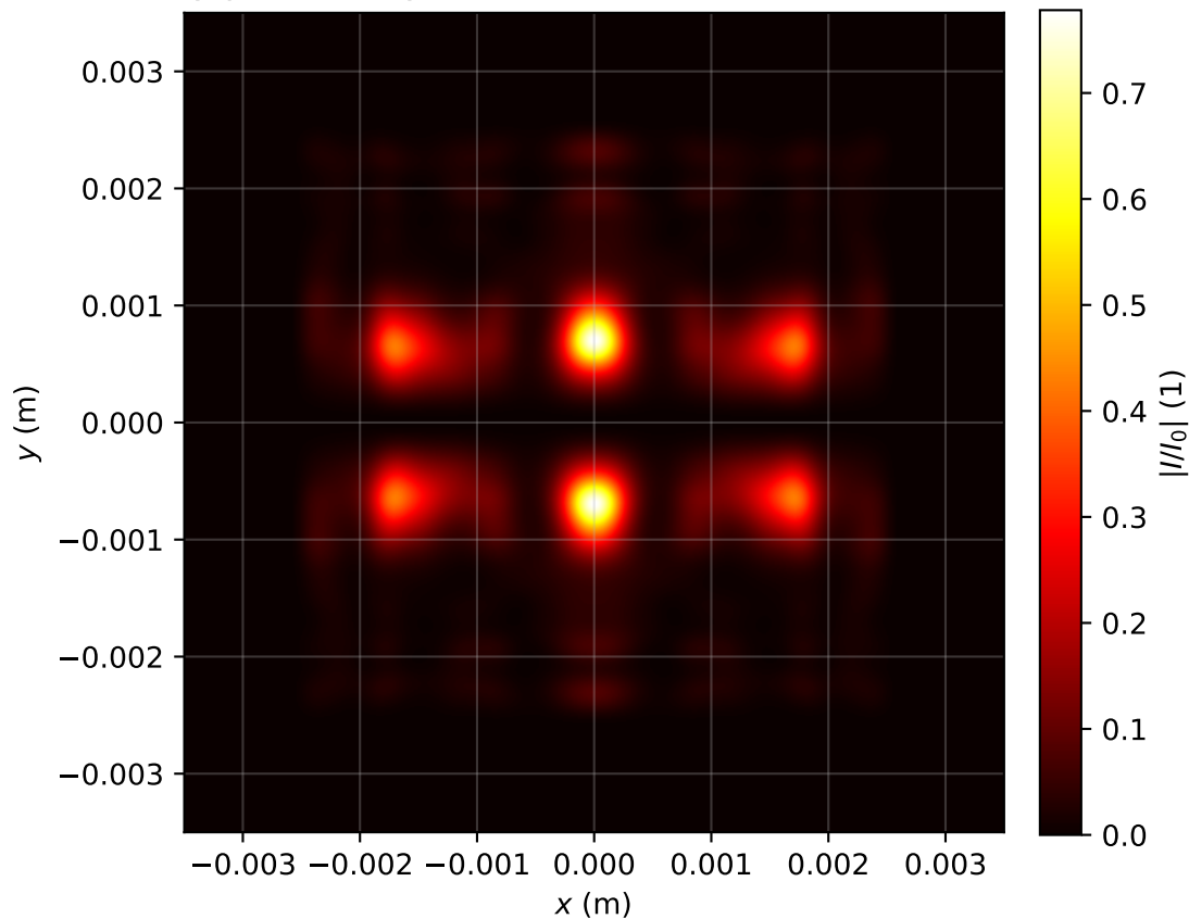
Intensity profile I(x, y, z = 3.423)/I_0 , P_{in}=5.0P_{cr} , artificial time
